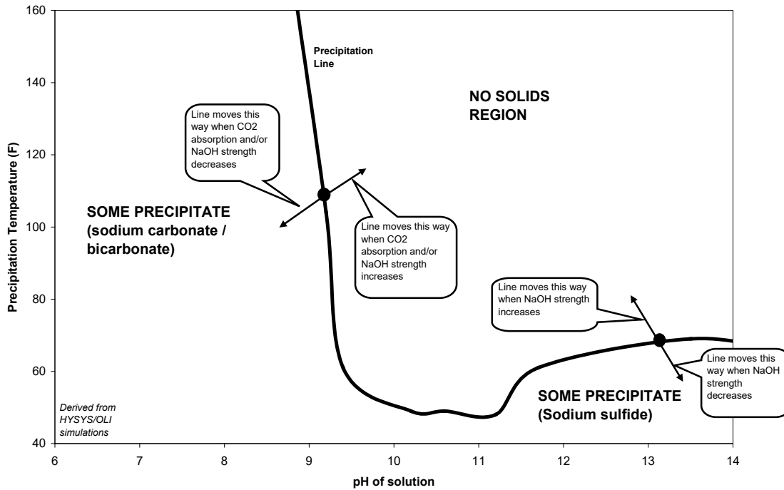
Figure 8. Example of General Trends of Solubility Limits for a Particular Scrubbing Solution. Systems where the gas contains both H 2 S and CO 2 .
