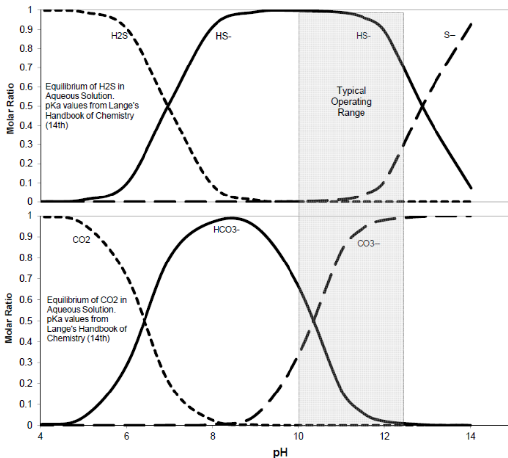
Figure 7. CO 2 and H 2 S Speciation in Aqueous Solution (based on pKa values from Ref. 1)
