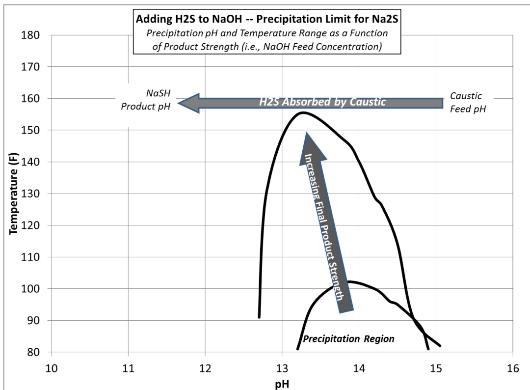
Figure 9. Example of General Trends of the Solubility Limit for a Particular Scrubbing Solution. System where the gas contains H 2 S (no CO 2 ) showing the solubility limit of Na 2 S.
